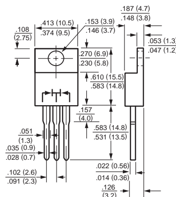
TO-220
