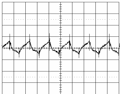
Output voltage ripple (20mV/div.) at: T_{ref} = +25^\circ\text{C} , I_O = 6\text{ A} resistive load, V_i = 5.0\text{ V} . Time scale: 1 \mu\text{s} /div. See the filter in the Output ripple and noise section (EMC Specification).
