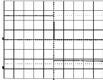
Shut-down enabled by disconnecting V_i at: T_{ref} = +25^\circ\text{C} , I_O = 6\text{ A} resistive load, V_i = 3.3\text{ V} . Top trace: output voltage (1.0 V/div.). Bottom trace: input voltage (5 V/div.). Time scale: 20.0 ms/div.
