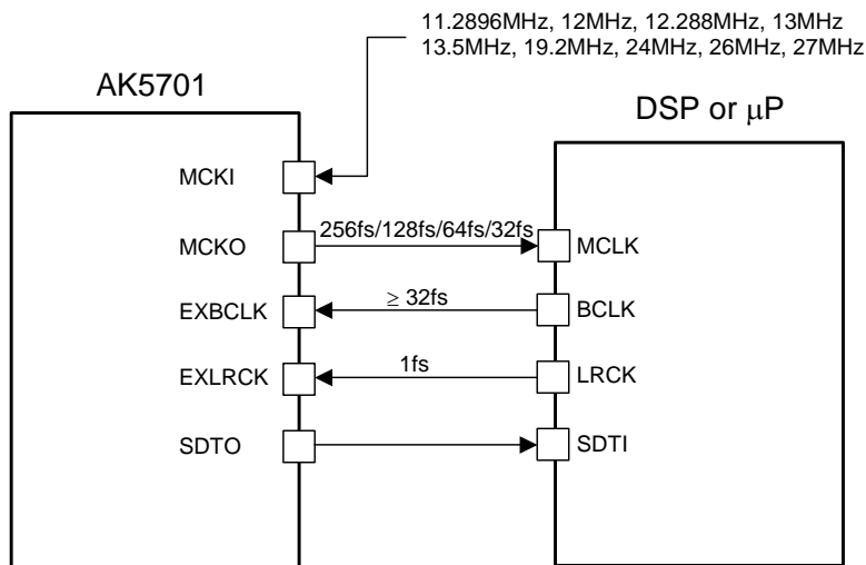
Figure 21. PLL Slave Mode 2 (PLL Reference Clock: MCKI pin)
