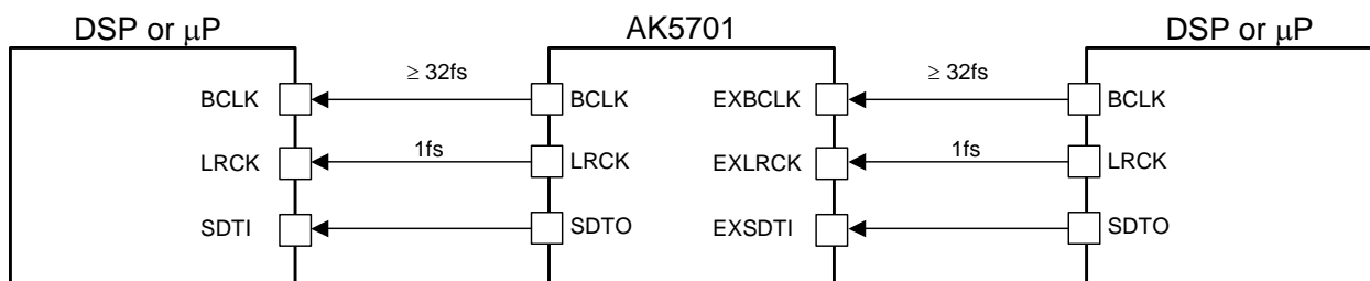
Figure 24. Bypass Mode
