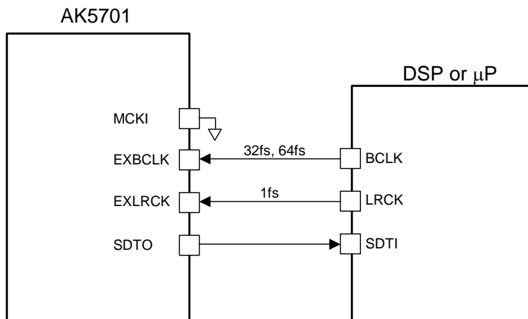
Figure 20. PLL Slave Mode 1 (PLL Reference Clock: EXLRCK or EXBCLK pin)
