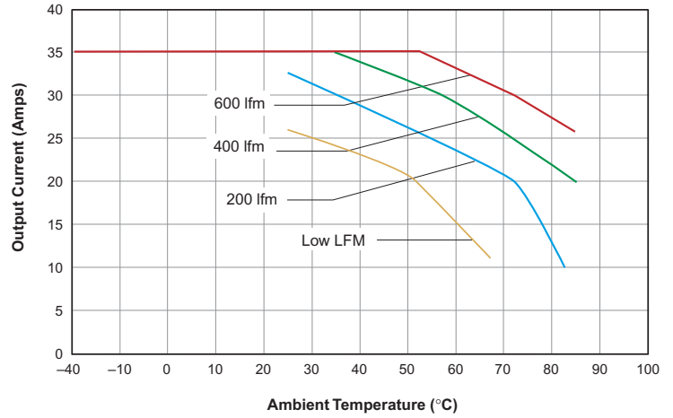
USQ-3.3/35-D48: Output Current vs. Ambient Temperature (Transverse air flow, pin 1 to pin 3; VIN = 48V, no heat sink.)
