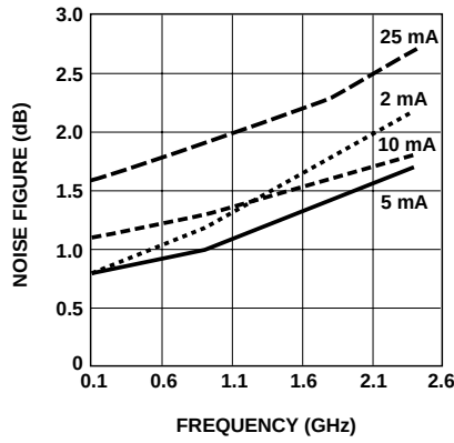
Figure 2. AT-41511 and AT-41533 Minimum Noise Figure vs. Frequency and Current at V_{CE} = 5 V.
