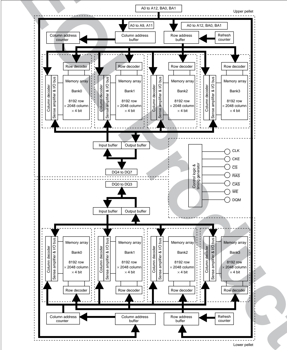
Block Diagram (HM5257805B)
