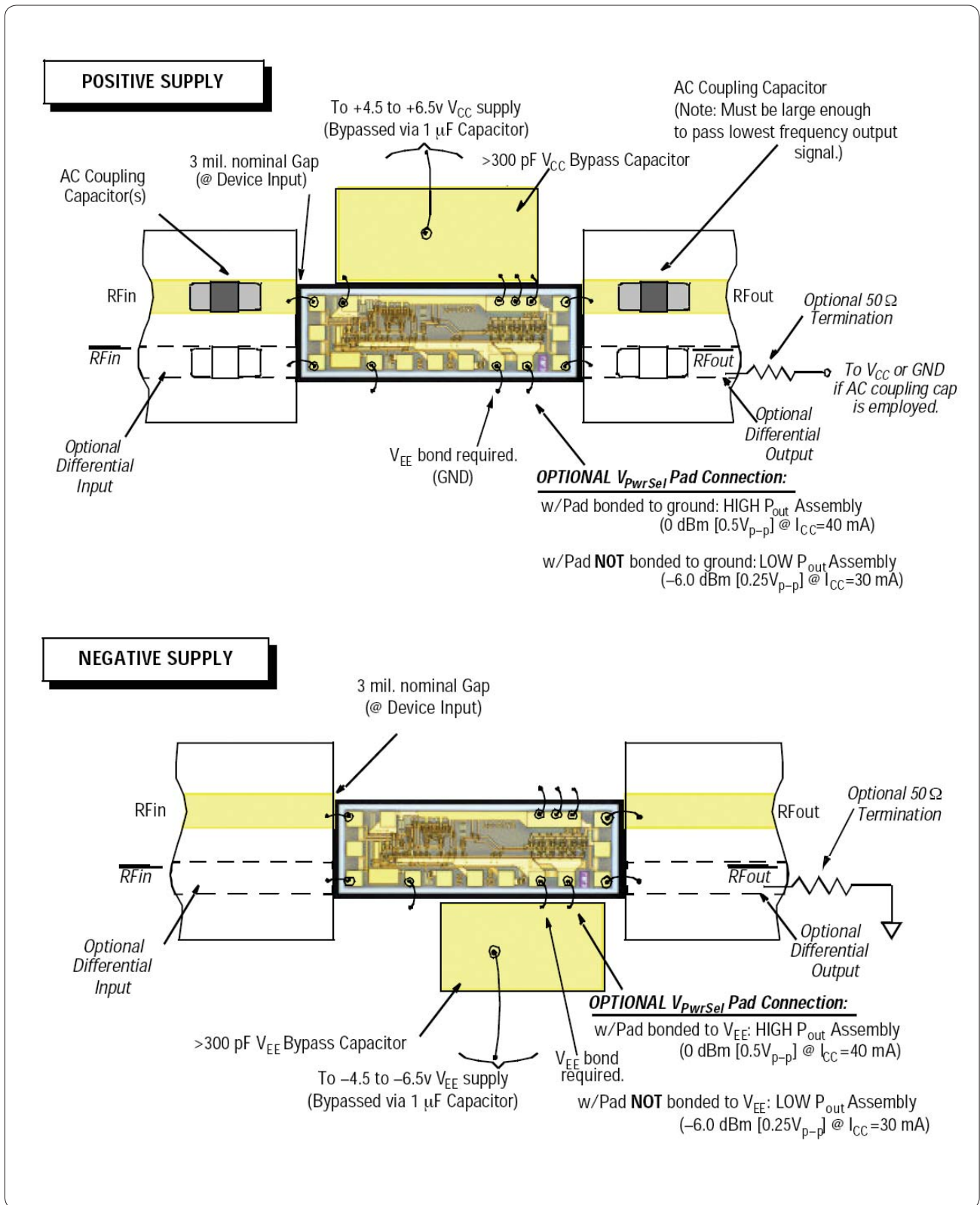
Figure 3. Assembly diagrams
