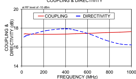
ADC-18-4-75 COUPLING & DIRECTIVITY
