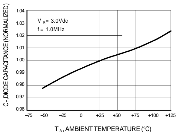
Figure 3. Diode Capacitance
