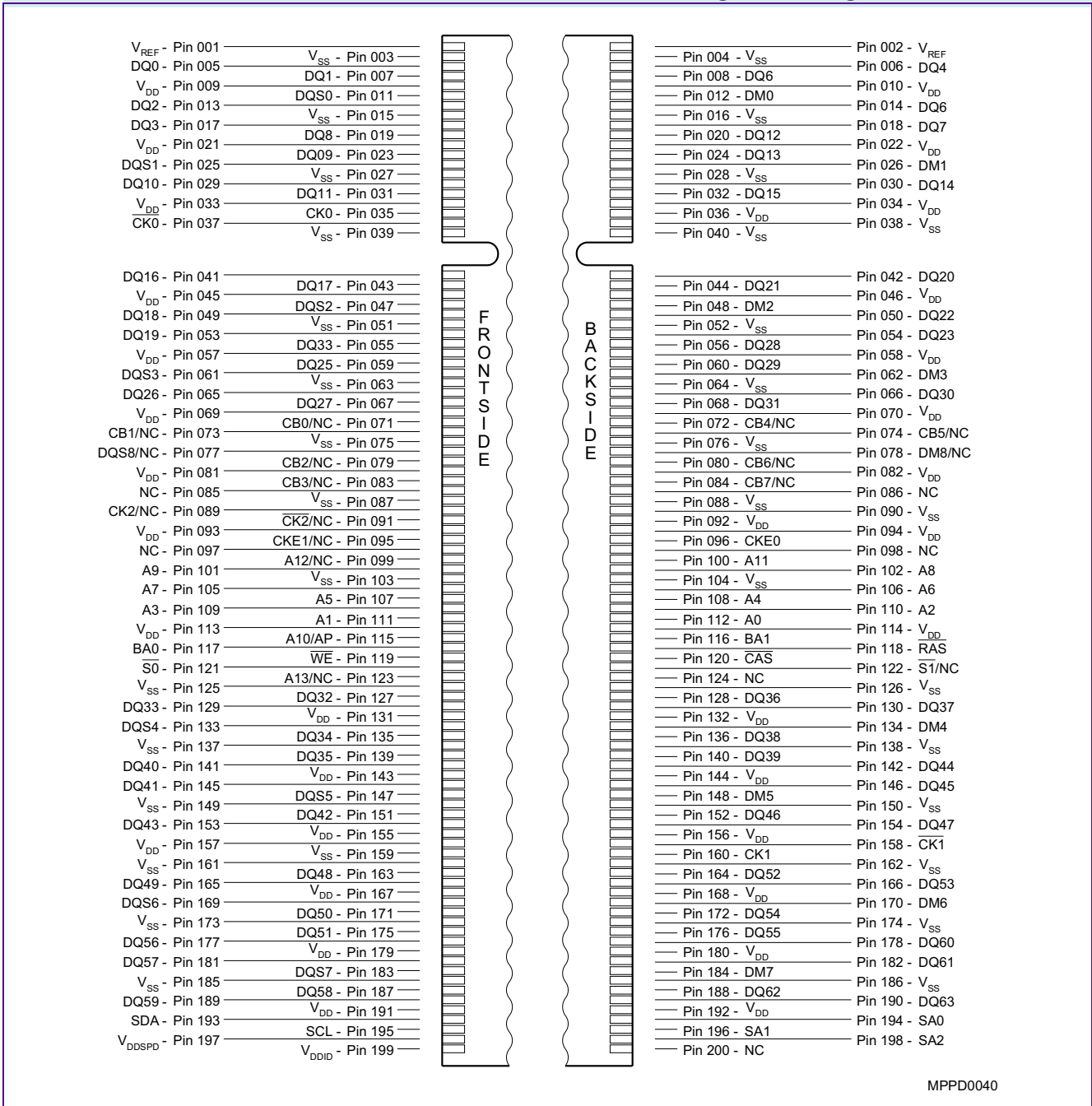
FIGURE 1 Pin Configuration Diagram 200-Pin SO-DIMM
