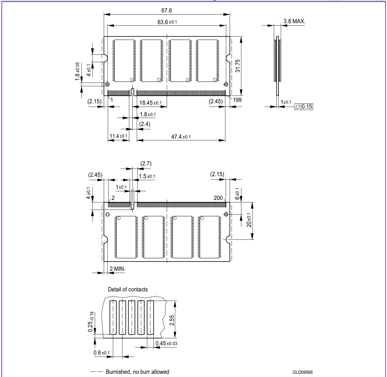
FIGURE 2 Package Outline SO-DIMM Raw Card A (L-DIM-200-6)
