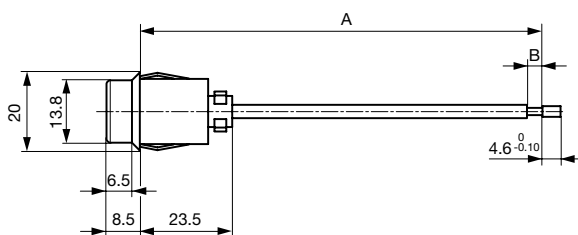
Type A (Snap-in mounting)
