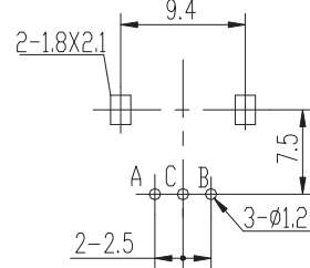
PCB LAYOUT
