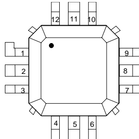
Figure 3: Pin Layout
