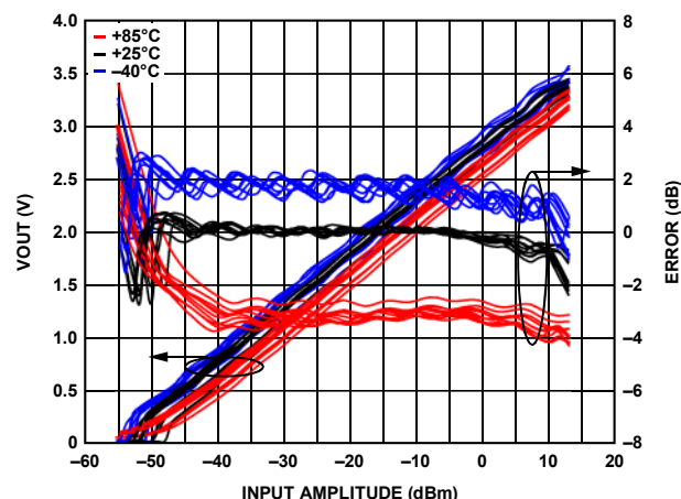
Figure 23. VOUT and Law Conformance vs. Input Amplitude for 15 Devices, Frequency 2800 MHz, Sine Wave, Temperatures: -40°C, +25°C, and +85°C, No Temperature Compensation, Single-Ended Drive, See Figure 50
