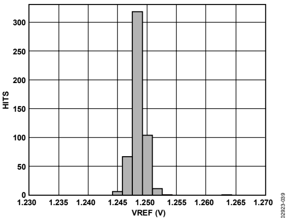
Figure 39. VREF Distribution
