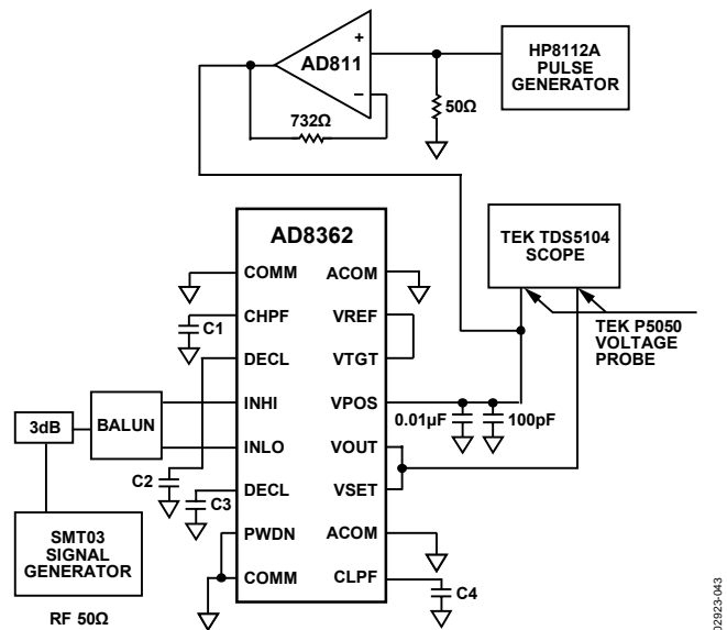
Figure 43. Response Measurement Setup for Gated Supply
