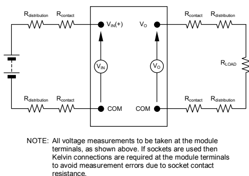
Figure 27. Output Voltage and Efficiency Test Setup.
