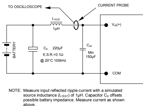
Figure 25. Input Reflected Ripple Current Test Setup.
