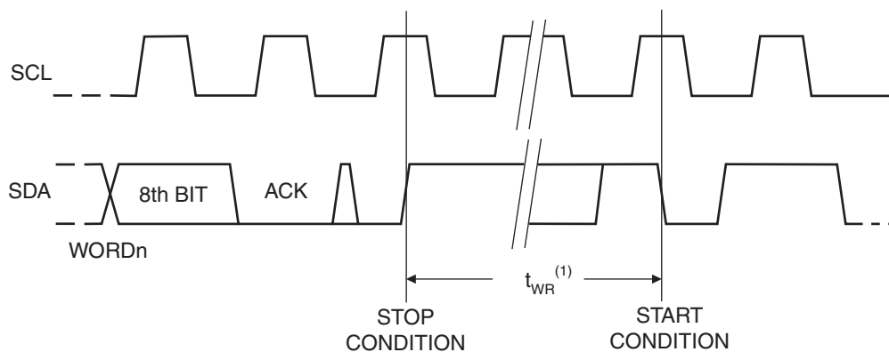
Figure 7-2. Write Cycle Timing. SCL: Serial Clock, SDA: Serial Data I/O
