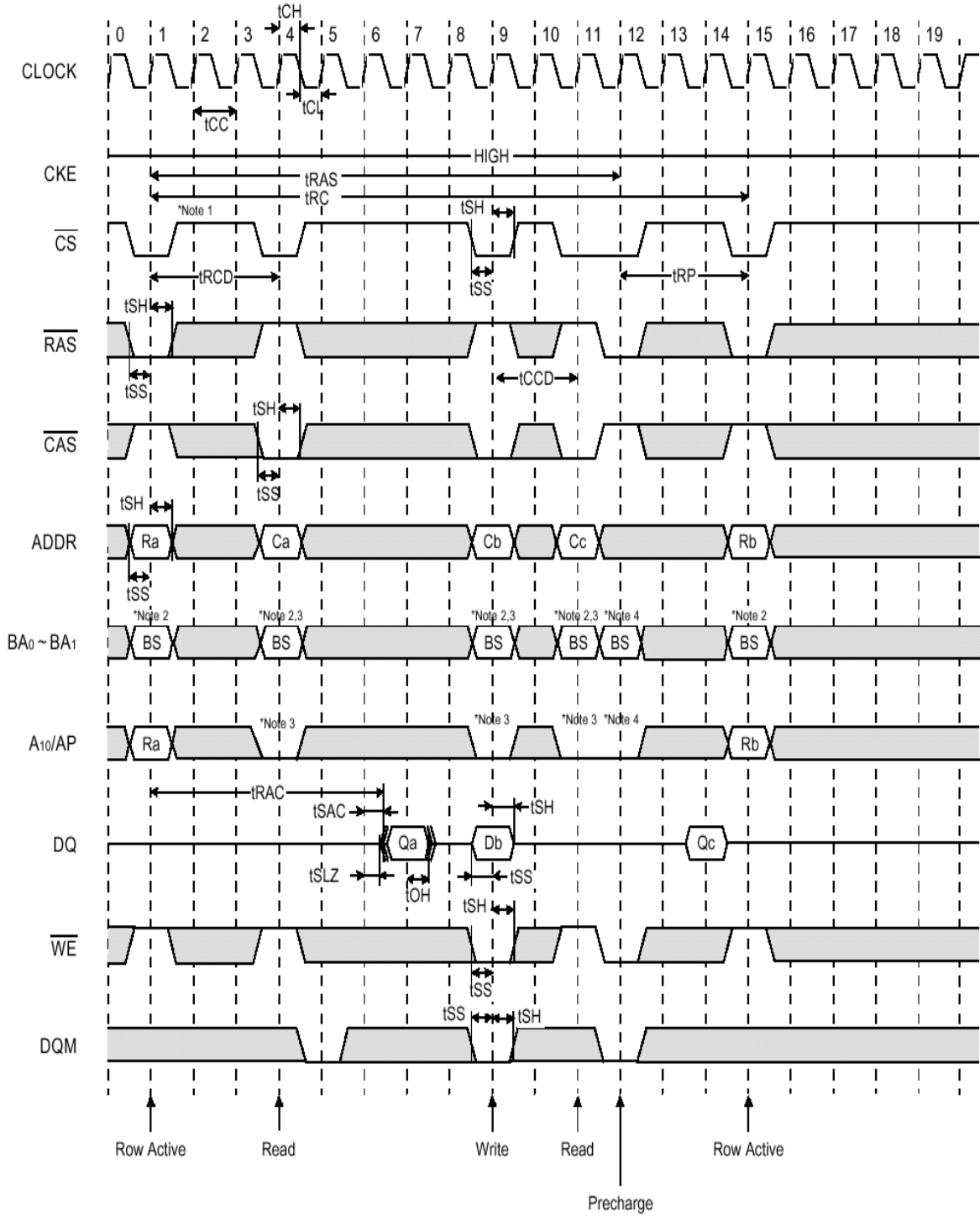
Single Bit Read-Write-Read Cycle(Same Page) @CAS Latency=3, Burst Length=1
