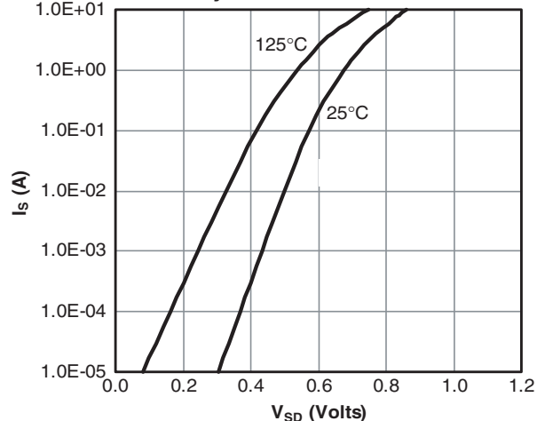
Body-Diode Characteristics
