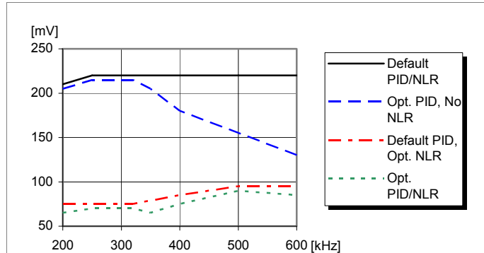
Load transient peak voltage deviation vs. frequency. Step-change (5-15-5 A). T_{P1} = +25^\circ C , V_I = 12 V , V_O = 1.0 V , C_O = 470 \mu F .
