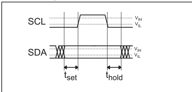
SMBus timing diagram
