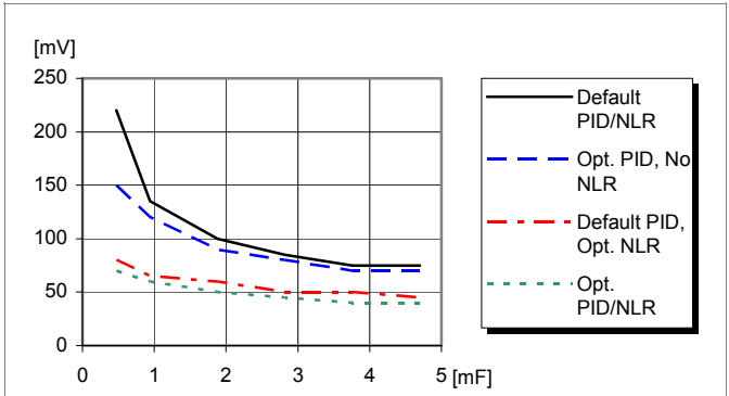
Load transient peak voltage deviation vs. decoupling capacitance. Step-change (5-15-5 A). Parallel coupling of capacitors with 470 \mu F / 10 m \Omega , T_{P1} = +25^\circ C , V_I = 12 V , V_O = 3.3 V , f_{sw} = 320 kHz , di/dt = 2 A/\mu s
