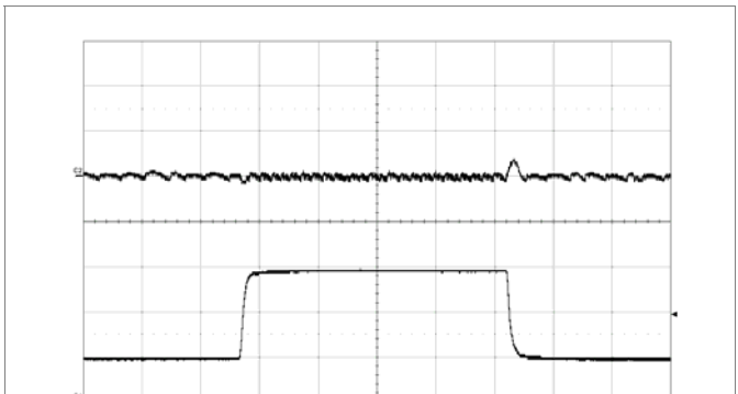
Output voltage response to load current step-change (5-15-5 A) at: T_{P1} = +25^\circ C , V_I = 12 V , V_O = 1.0 V , di/dt = 2 A/\mu s , f_{sw} = 320 kHz , C_O = 470 \mu F . Default PID Control Loop and optimized NLR. Top trace: output voltage (200 mV/div.). Bottom trace: load current (5 A/div.). Time scale: (0.1 ms/div.).
