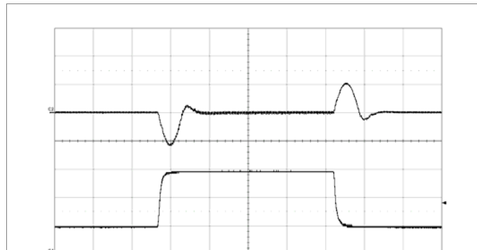
Output voltage response to load current step-change (5-15-5 A) at: T_{P1} = +25^\circ C , V_I = 12 V , V_O = 1.0 V , di/dt = 2 A/\mu s , f_{sw} = 320 kHz , C_O = 470 \mu F . Optimized PID Control Loop and no NLR. Top trace: output voltage (200 mV/div.). Bottom trace: load current (5 A/div.). Time scale: (0.1 ms/div.).
