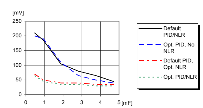
Load transient peak voltage deviation vs. decoupling capacitance. Step-change (5-15-5 A). Parallel coupling of capacitors with 470 \mu F / 10 m \Omega , T_{P1} = +25^\circ C , V_I = 12 V , V_O = 1.0 V , f_{sw} = 320 kHz , di/dt = 2 A/\mu s
