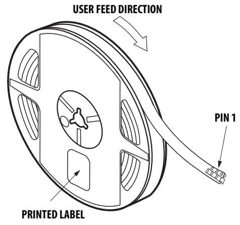
Figure 15. Reeling Orientation
