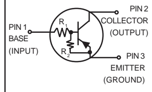
CASE 419, STYLE 3 SOT-323 (SC-70)
