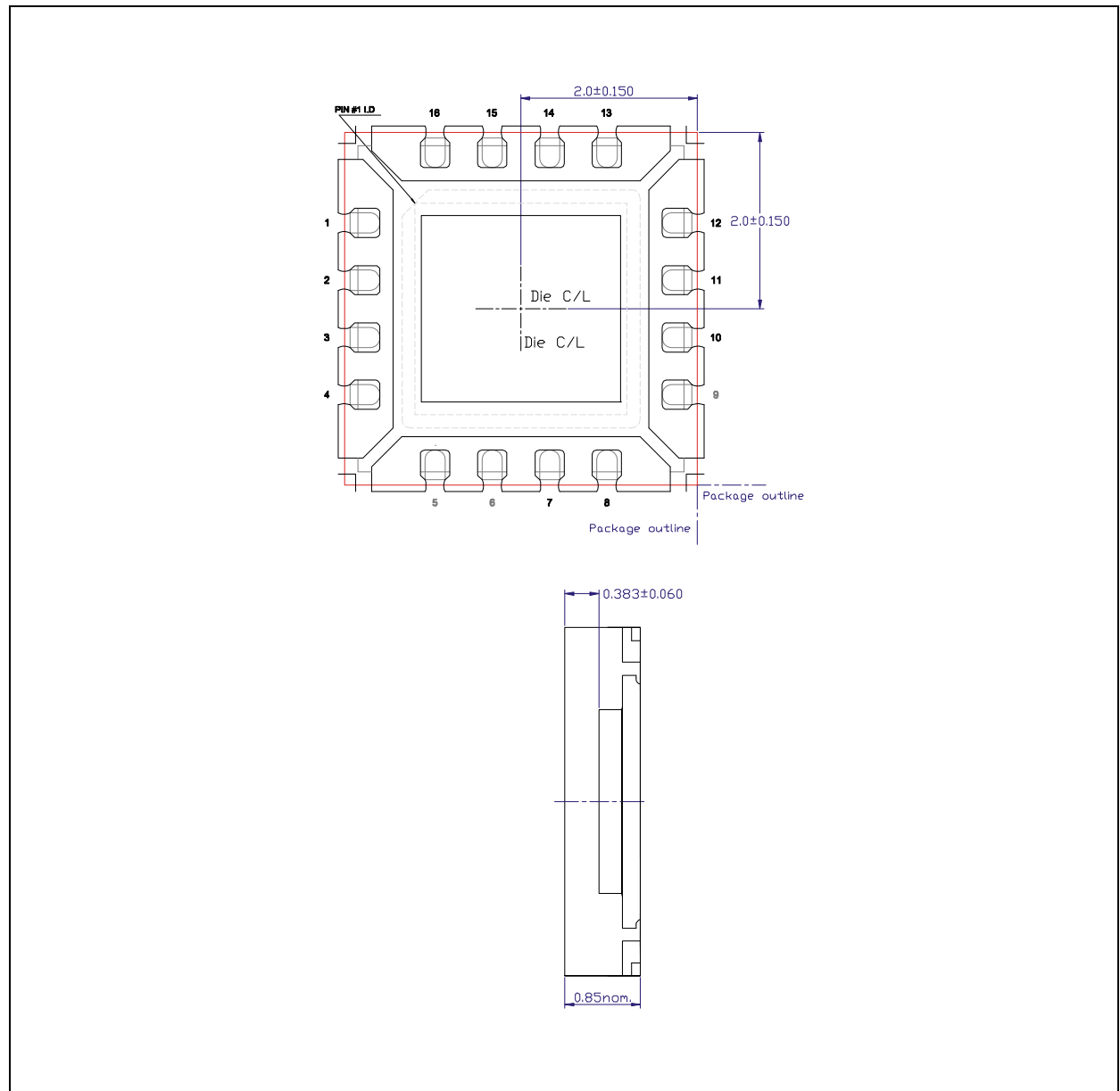
Figure 35: Vertical Cross Section of QFN 16-pin 4x4x0.85 mm package
