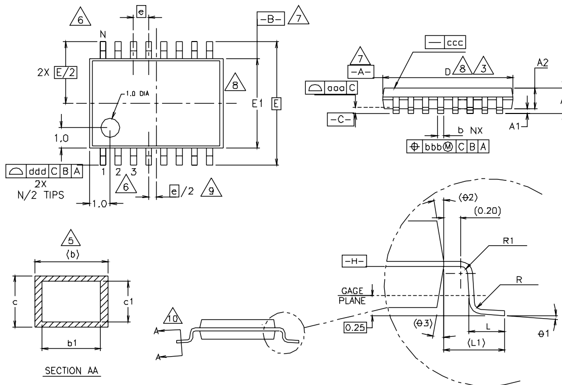
Figure 37. 20-pin TSSOP Package
