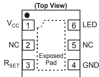
U-DFN3030-6
