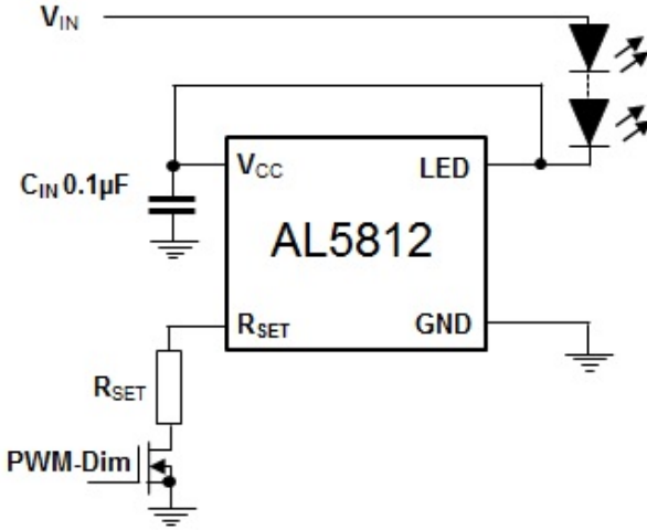
Figure 17 PWM Dimming
