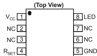
MSOP-8EP
