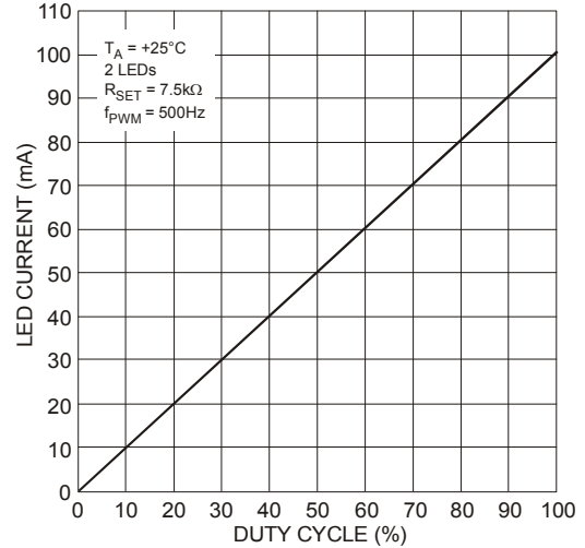
Figure 18 PWM Dimming Linearity
