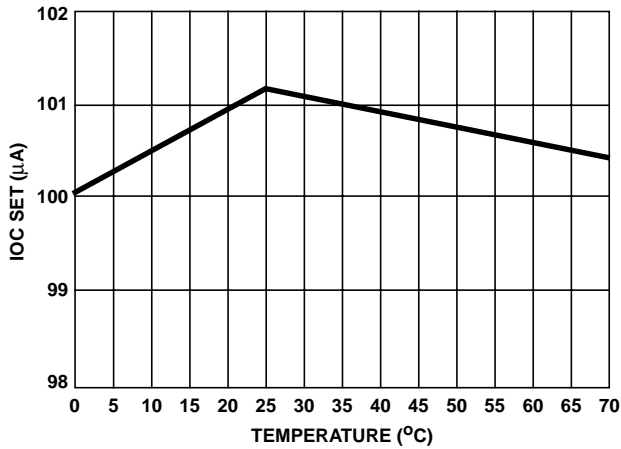
FIGURE 12. IOC SET vs TEMPERATURE
