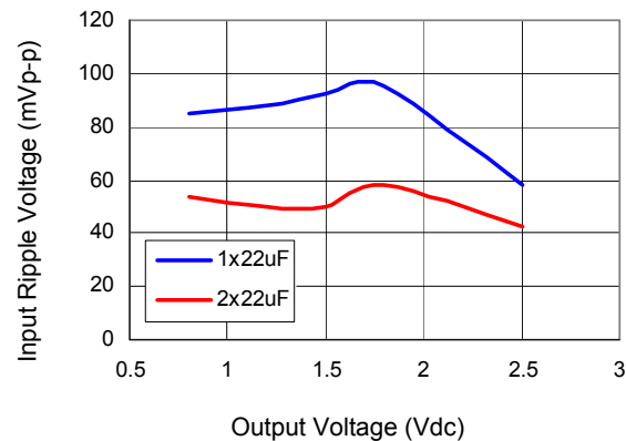
Figure 35. Input ripple voltage in mV, p-p for various output voltages with 1x22 μF or 2x22 μF ceramic capacitors at the input (6A load). Input voltage is 3.3V.
