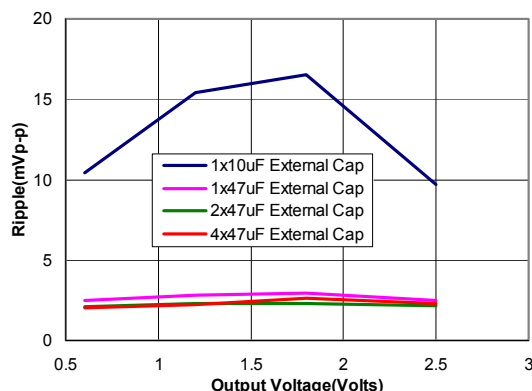
Figure 37. Output ripple voltage for various output voltages with external 1x10 \mu F, 1x47 \mu F, 2x47 \mu F or 4x47 \mu F ceramic capacitors at the output (6A load). Input voltage is 3.3V.
