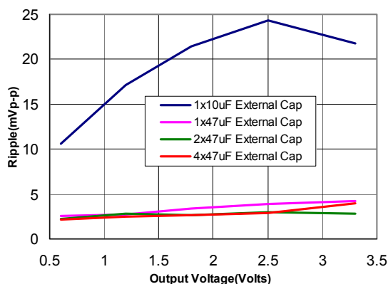
Figure 36. Output ripple voltage for various output voltages with external 1x10 \mu F, 1x47 \mu F, 2x47 \mu F or 4x47 \mu F ceramic capacitors at the output (6A load). Input voltage is 5V.
