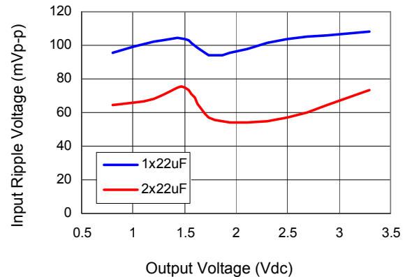
Figure 34. Input ripple voltage for various output voltages with 1x22 μF or 2x22 μF ceramic capacitors at the input (6A load). Input voltage is 5V.
