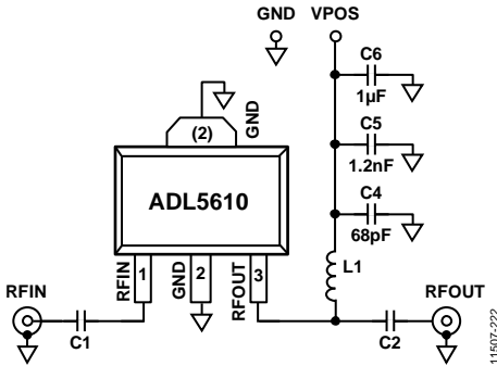
Figure 26. Basic Connections
