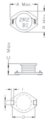
Figure 4 (Case Size: 50)
