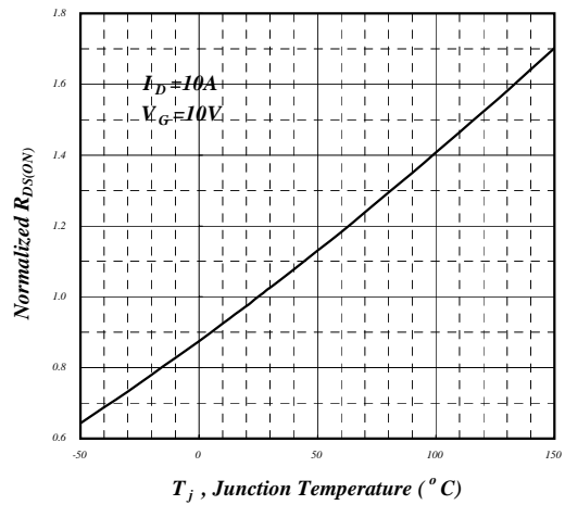
4. Normalized On-Resistance v.s. Junction Temperature
