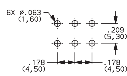
PIN LAYOUT
