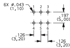
PC MOUNTING
