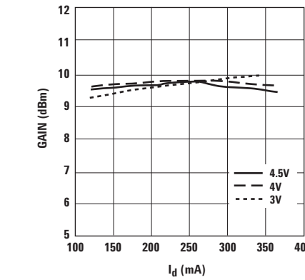
Figure 16. Small Signal Gain vs I_{ds} and V_{ds} at 3.9 GHz.
