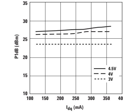
Figure 13. P1dB vs. I_{dq} and V_{ds} at 3.9 GHz.
