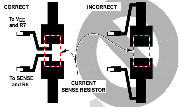
FIGURE 30. SENSE RESISTOR LAYOUT GUIDELINES
