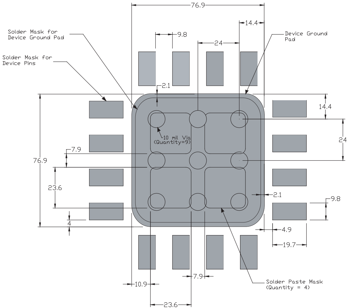
Figure 32: Recommended PCB Layout (all units are in mils)
