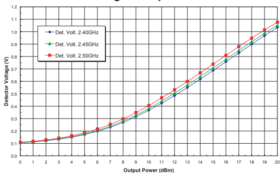
Figure 8: Tx Path Detector Voltage vs. Output Power Across Freq ( T_A = +25^\circ\text{C} , V_{CC} = +3.6\text{ V} ) 802.11g 54 Mbps OFDM
