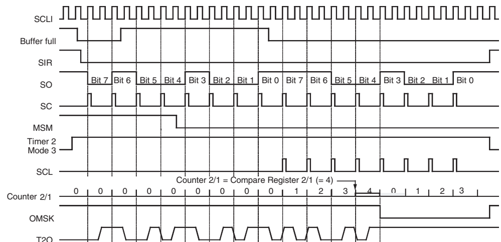
Figure 24-5. Manchester Modulation 2
