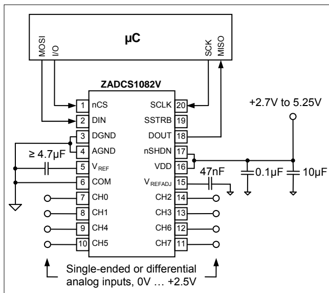
Figure 4: Basic application schematic for ZADC1082V
