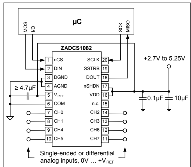
Figure 5: Basic application schematic for ZADC1082
