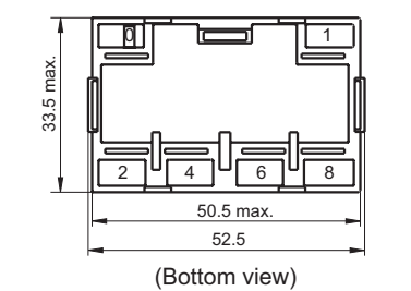
HF116F-1/□□□□-□-A-2H-□
