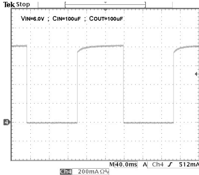
Short Circuit-Current
