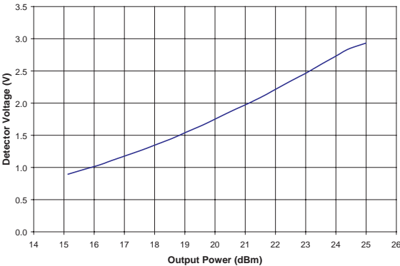
Figure 7: Detector Voltage vs. Output Power (T C = +25 °C, V CC = +6.0 V, V BIAS = +3.0 V, f = 3.7 GHz, 54 Mbps OFDM Modulation)
