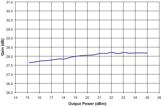
Figure 3: Gain vs. Output Power (T C = +25 °C, V CC = +6.0 V, V BIAS = +3.0 V, f = 3.7 GHz, 54 Mbps OFDM Modulation)
