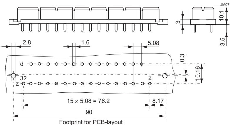
Fig. 9c HZZ00117-G (STV-H15-FP/CO), press fit pins, foot print
