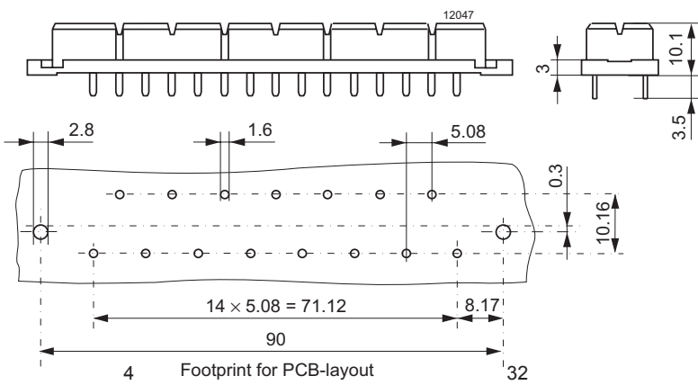
Fig. 9a HZZ00112-G (STV-H15-FB/CO), solder pins, foot print.
