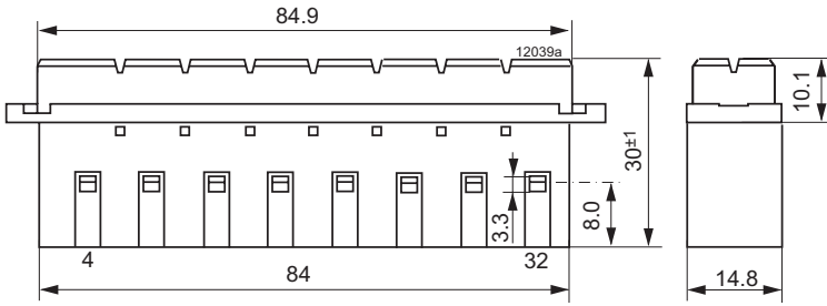
Fig. 8 HZZ00107-G (STV-H15-FSR-G), screw terminals, no coding, max torque 26.6 Ncm HZZ00106-G (STV-H15-F/CO-G), Faston terminals 6.3 × 0.8 mm (identical dimensions, but not shown). The orientation of the faston terminals can be horizontal or vertical, depending on supplier.
