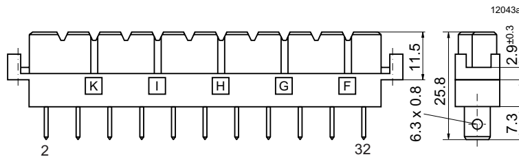
Fig. 3 HZZ00104-G (STV-H11-FS/CO), faston terminals 6.3 \times 0.8 mm, solderable (short moulding)
