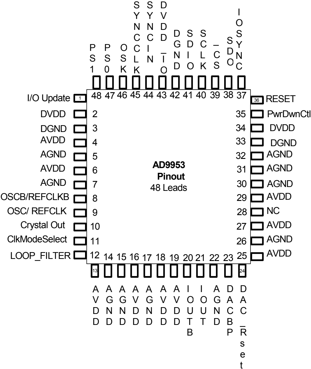
Figure 1 AD9953 Pinmap
