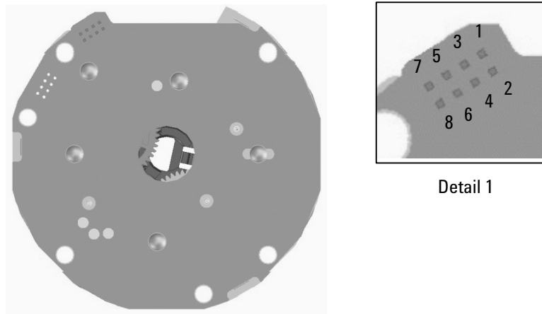
Figure 8. Pin Configuration
