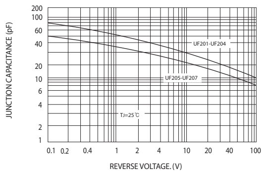
FIG.6-TYPICAL JUNCTION CAPACITANCE
