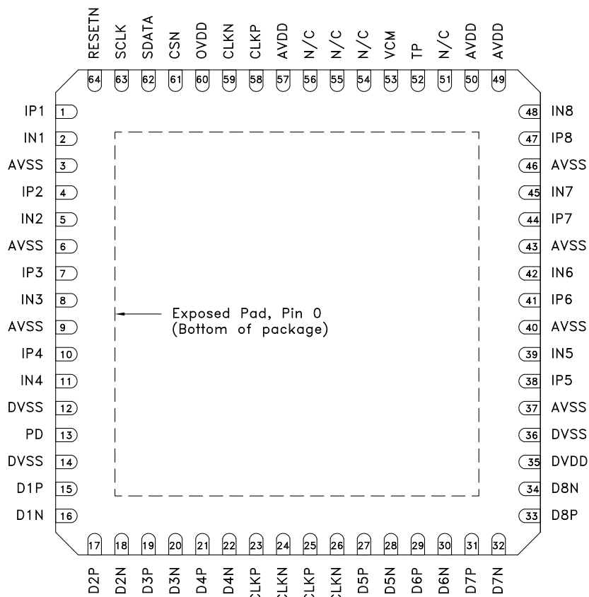
Figure 2. Package Diagram
