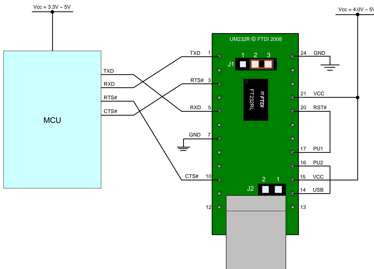
Figure 7.2 Self-Powered Configuration
