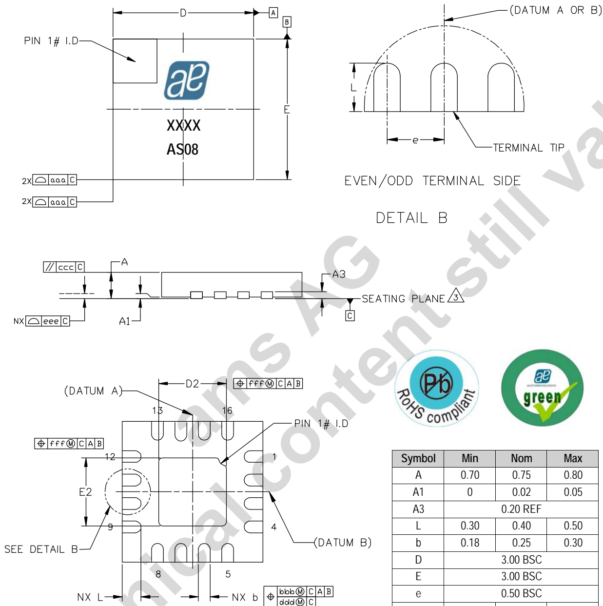
Figure 29. TQFN-16 (3x3mm)
