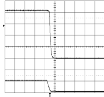
Shut-down enabled by disconnecting V_i at: T_{ref} = +25^\circ\text{C} , I_o = 1.5\text{ A} resistive load, V_i = 53\text{ V} . Top trace: output voltage (0.5 V/div.). Bottom trace: input voltage (50 V/div.). Time scale: 2 ms/div.
