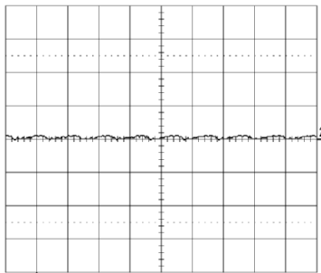
Output voltage ripple (20mV/div.) at: T_{ref} = +25^\circ\text{C} , I_o = 1.5\text{ A} resistive load, V_i = 53\text{ V} . Time scale: 2 \mu\text{s} /div. See the filter in the Output ripple and noise section (EMC Specification).
