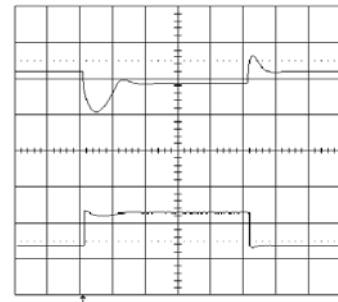
Output voltage response to load current step-change (0.38-1.13-0.38 A) at: T_{ref} = +25^\circ\text{C} , V_i = 53\text{ V} . Top trace: output voltage (200mV/div.). Bottom trace: load current (1 A/div.). Time scale: 0.1 ms/div.
