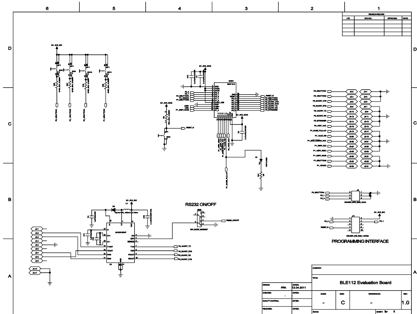
Figure 5: BLE112 Development Board Schematic (3/3)
