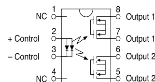
LCA210 Pinout
