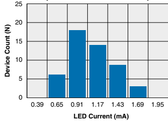
IAB110P - FormA Typical I F for Switch Dropout (N=50 Ambient Temperature = 25°C) (Load Current = 100mADC)
