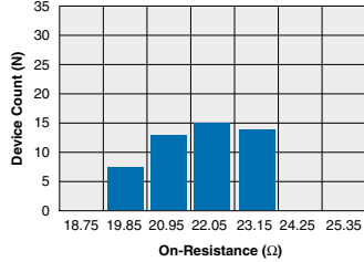
IAB110P - FormA Typical On-Resistance Distribution (N=50 Ambient Temperature = 25°C) (Load Current = 100mADC, I F =5mADC)
