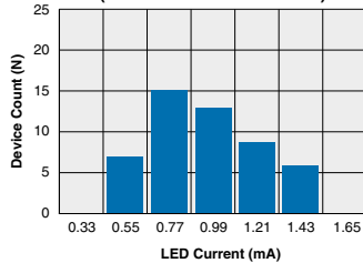
IAB110P - FormB Typical I F for Switch Operation (N=50 Ambient Temperature = 25°C) (Load Current = 100mADC)
