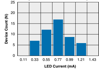
IAB110P - FormB Typical I F for Switch Dropout (N=50 Ambient Temperature = 25°C) (Load Current = 100mADC)
