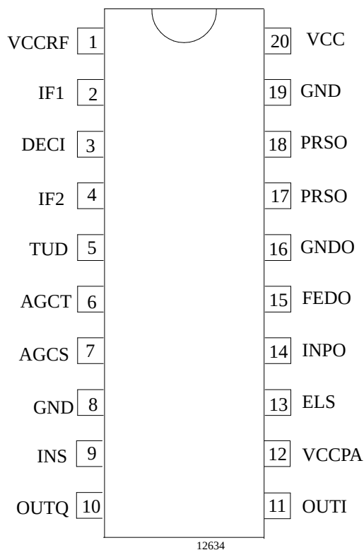
Figure 2. Pinning
